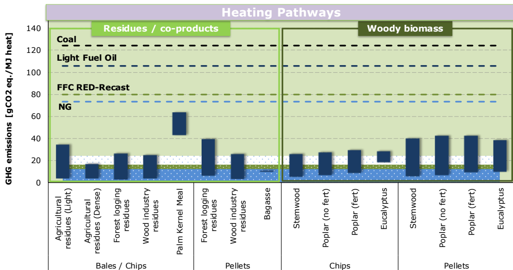
Figure 7.11. GHG emissions from pathways for the production of heating from various biomass feedstocks
