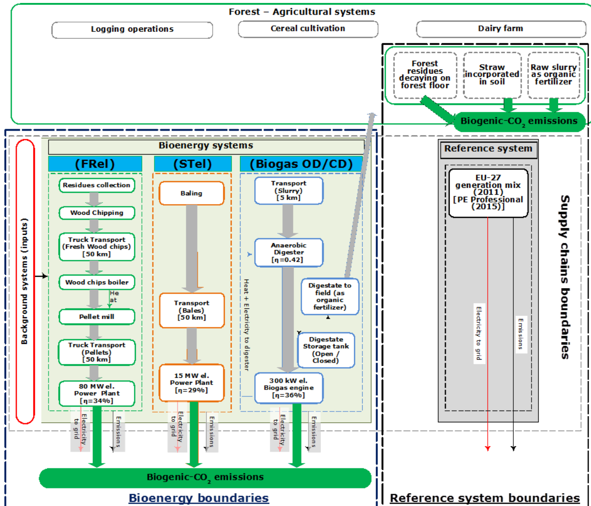
Figure 7.15. System boundaries for the three systems considered
