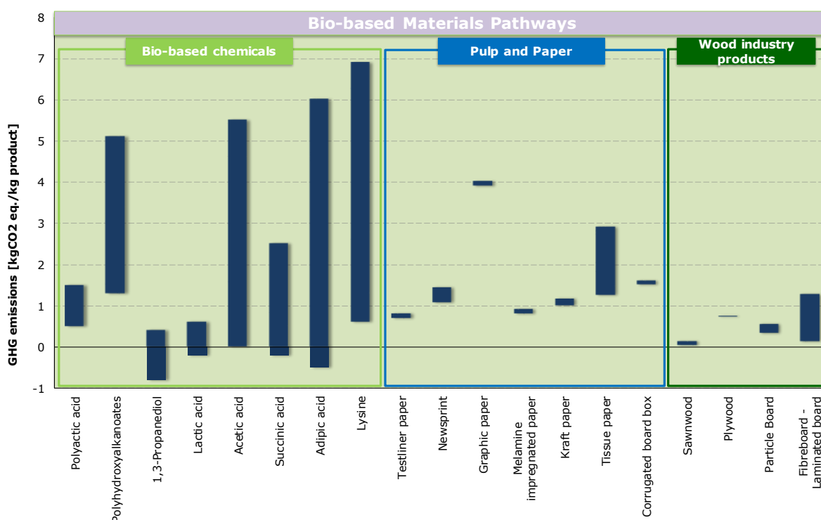
Figure 7.13. GHG emissions from pathways for the production of bio-based chemicals, pulp and paper and wood industry products
