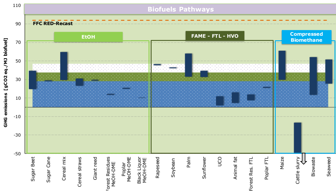
Figure 7.12. GHG emissions from pathways for the production of biofuels for transport from various biomass feedstocks
