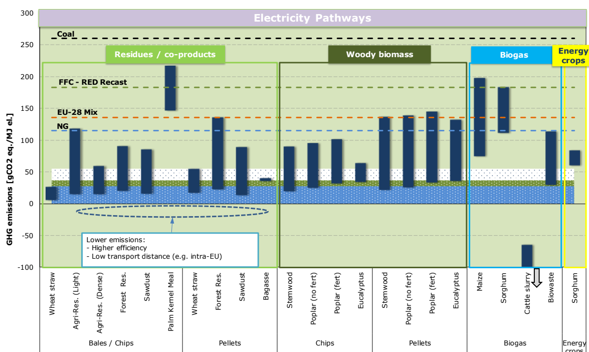
Figure 7.10. GHG emissions from pathways for the production of electricity from various biomass feedstocks
