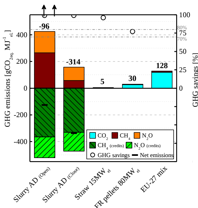
Figure 7.16. Supply chain GHG emissions for bioenergy and EU-27 mix
